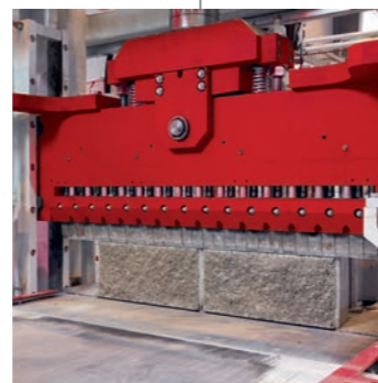
34 Splitting machines
