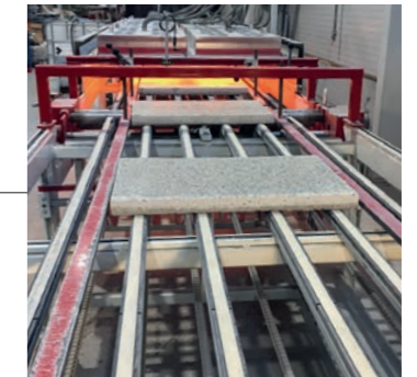
28 Coating line
